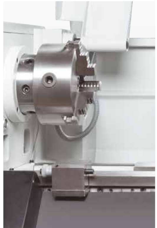
Micrometer bed stop ensures repeatability
